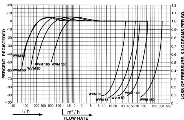
Curves Accuracy and Head Loss
